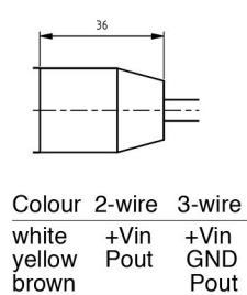
Fig. 17 - Cable connection IP68
